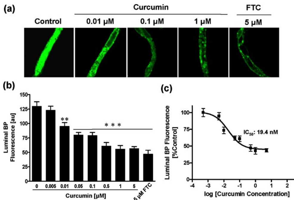
Fig. 1. Curcumin inhibits the activity of ABCG2 in rat brain capillaries. a Isolated, functionally intact rat brain capillaries were incubated with 2 \mu M BODIPY® FL prazosin in the absence (control) or presence of varying concentrations of curcumin (middle three panels) and 5 \mu M FTC at room temperature for 1 h and the images were acquired as described in “Materials and Methods”. Representative images from a single experiment from three individual experiments are shown here. b Luminal BODIPY® FL prazosin fluorescence in capillaries in the presence and absence of varying concentrations of curcumin was quantitated as described in “Materials and Methods” using Image J software and plotted as a function of curcumin concentrations. Statistical comparison: **, significantly lower than control capillaries, P < 0.01 ; ***, significantly lower than control capillaries, P < 0.001 . c Non-linear regression curve; data are plotted on a logarithmic scale. Each data point represents the luminal BODIPY® FL prazosin fluorescence mean value from ten capillaries (pooled capillary tissue from ten rats of a single preparation); variability is given by SEM bars. Units are arbitrary fluorescence units (scale 0–255).
