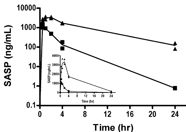
Fig. 3. Curcumin enhances plasma concentration of sulfasalazine in mice. Wild-type animals were pretreated with a single oral dose of curcumin (400 mg/kg) or vehicle for 1 h and all animals received a single oral dose of SASP (20 mg/kg). Line represents the average ( N=2 /time point). Blood collected by cardiac puncture and the concentration of SASP was detected by LC-MS/MS as described in “Materials and Methods”. The main graph represents the log plasma concentration of SASP (Y-axis) with respect to time (X-axis) in vehicle treated (squares) or curcumin and SASP (triangles) treated mice. Inset shows the SASP concentrations on Y-axis in linear scale.
