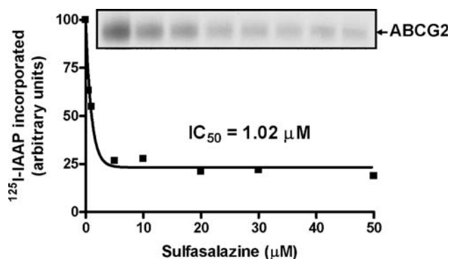
Fig. 2. Sulfasalazine inhibits the photolabeling of ABCG2 with [ 125 I]-IAAP binding. Crude membranes (500 \mu g/ml) from MCF-7 FLV1000 cells were incubated with 0–50 \mu M of SASP for 5 min at 21–23°C in 50 mM Tris-HCl, pH 7.5. 3–6 nM [ 125 I]-IAAP (2,200 Ci/mmol) was added and incubated for an additional 5 min under subdued light. The samples were then illuminated with a UV lamp (365 nm) for 10 min and were processed as described in “Materials and Methods”. A representative autoradiogram from one experiment is shown and similar results were obtained in two additional experiments. The arrow shows the position of the ABCG2 band. The incorporation of [ 125 I]-IAAP (from autoradiogram, Y-axis) into the ABCG2 (squares) band was quantified by estimating the radioactivity of this band plotted as a concentration of SASP using the software GRAPHPAD PRISM 2.0, as described previously (19).
