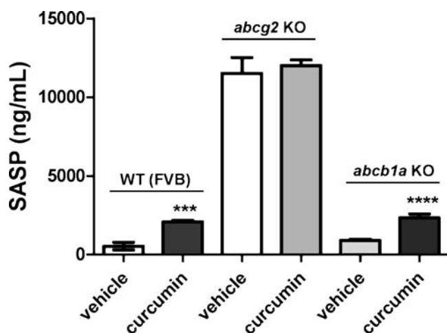
Fig. 4. Effect of curcumin on the plasma concentration of sulfasalazine in abcb1a , and abcg2 knock-out mice. All animals were treated with a single oral dose of curcumin (400 mg/kg) for 1 h followed by a single oral dose of sulfasalazine (20 mg/kg). At a pre-determined time point (90 min), mice were anesthetized with isoflurane, and blood samples were obtained by cardiac puncture and transferred to heparinized tubes. The samples were centrifuged immediately at 3,000×g for 15 min, and plasma was collected and stored at -80°C until the time of LC-MS/MS analysis. N=5 /treatment. Data reported as mean±SD. Two way ANOVA was used to compare the effect of curcumin versus vehicle on SASP absorption in wild type (FVB), abcg2 -/- ( abcg2 KO), and abcb1a -/- ( mdr1a KO) mice. Using Bonferroni's post-hoc test, the effect of curcumin pretreatment significantly increased SASP concentration in the wild-type ( P<0.001 ) and mdr1a ( abcb1a -/- ; P<0.001 ) mice. However, there was no significant increase in SASP exposure in abcg2 -/- mice after curcumin pretreatment ( P>0.05 ). As previously reported, abcg2 genotype significantly influences SASP Cmax ( P<0.0001 ) (15).
